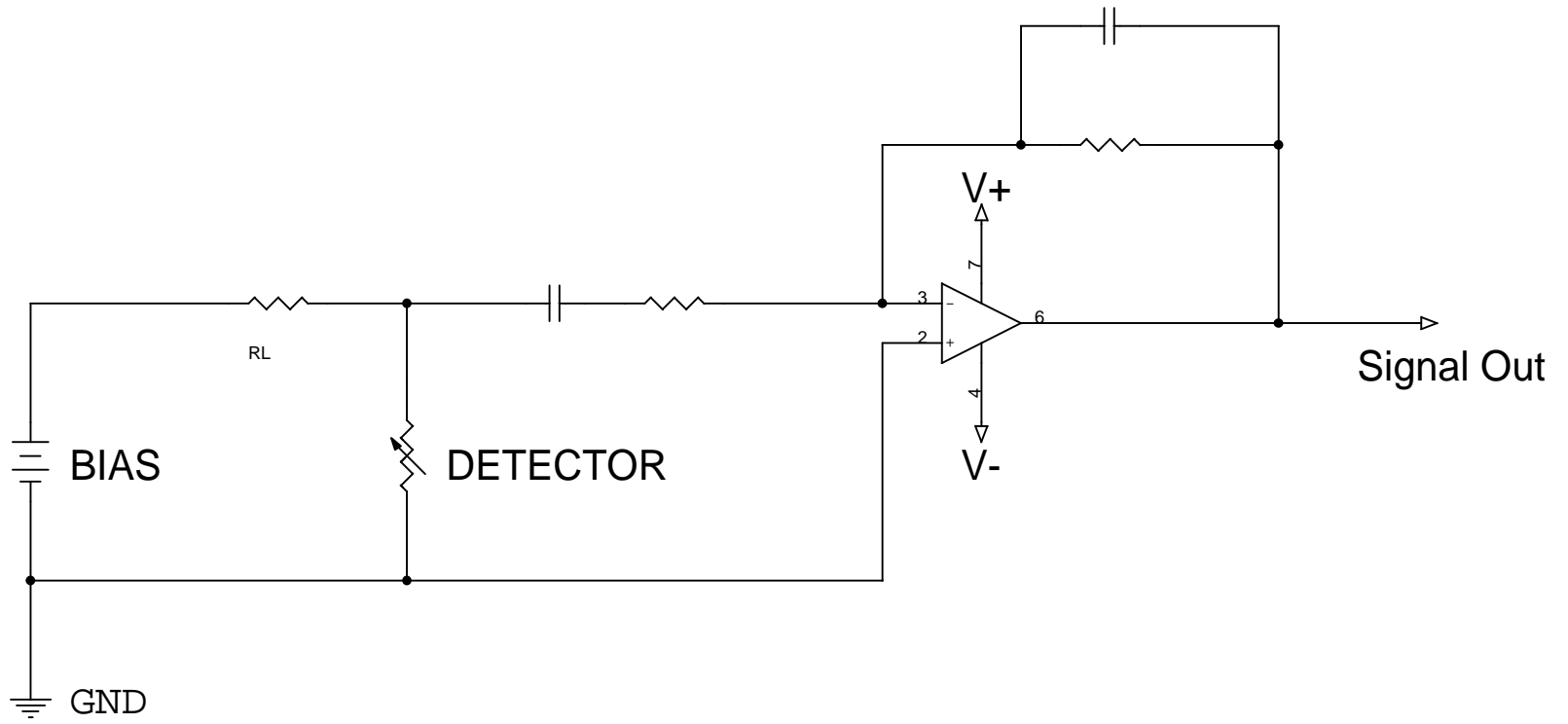
TYPICAL DETECTOR/PREAMPLIFIER CIRCUIT
